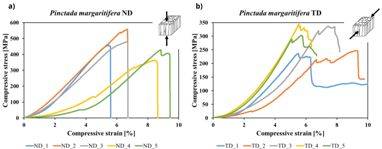
Fig. 2: Strain-stress curves of a P. margaritifera shell for compression tests along the depicted orientation. [2]
